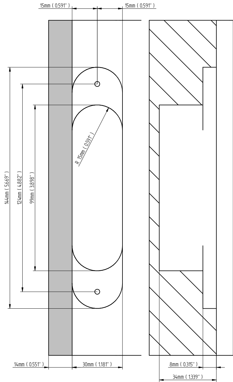
Template block frame
